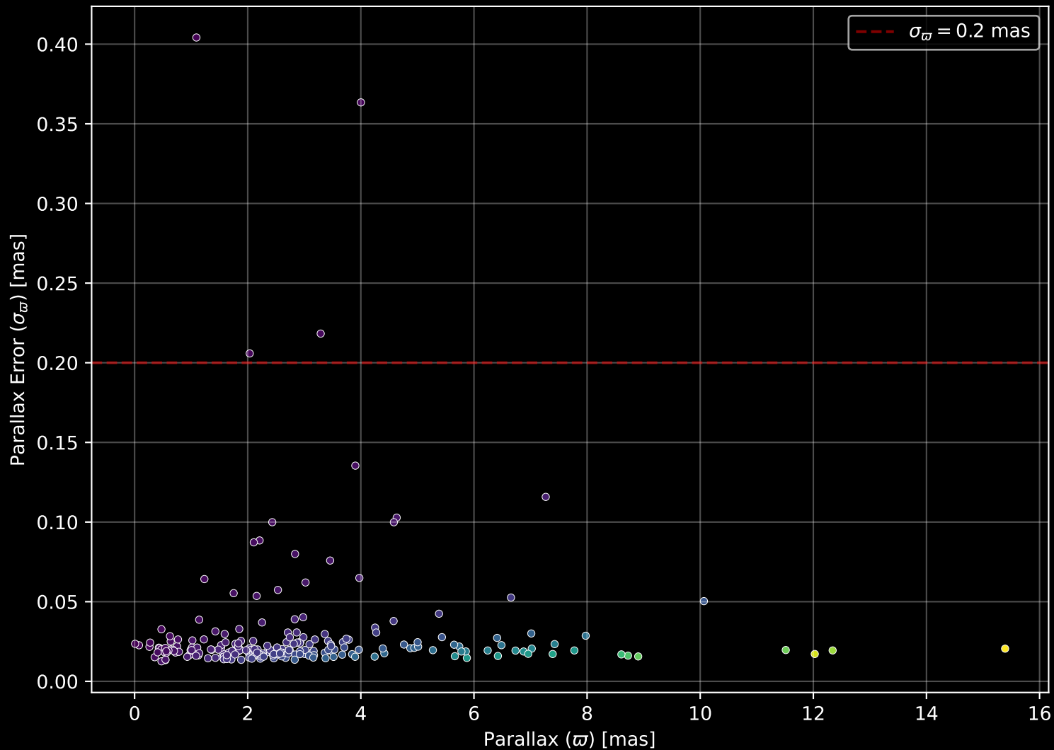
APOGEE DR17 Field: [160-60] Parallax Quality (n= 219)
