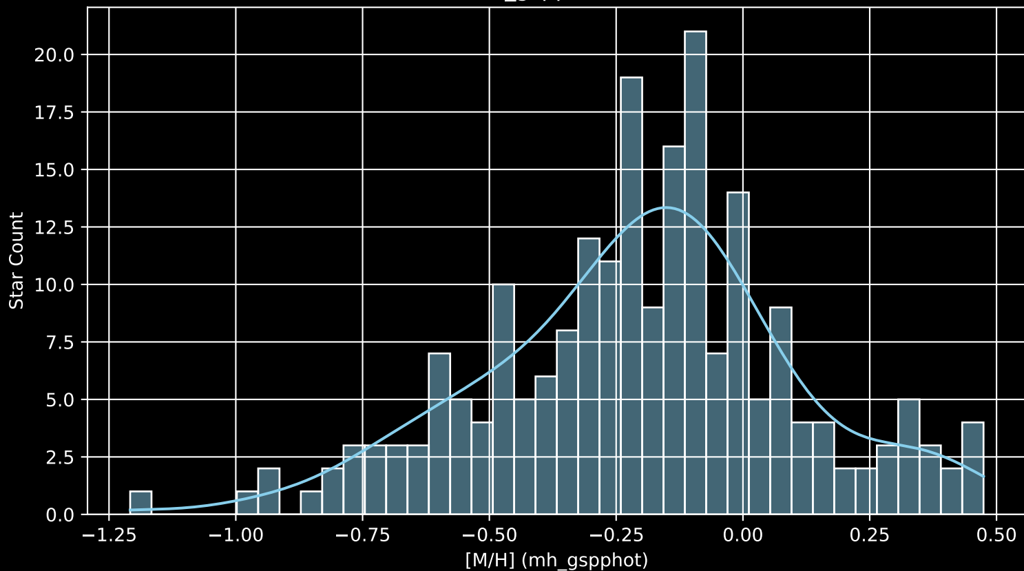
APOGEE DR17 Field: [160-60 [M/H] (mh_gspphot) (n= 216)
