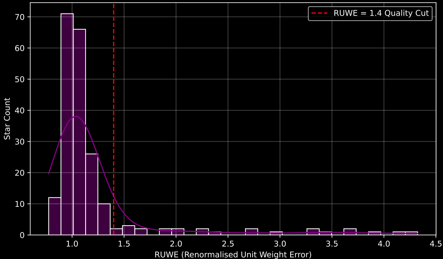
GAPOGEE DR17 Field [160-60] RUWE Distribution (n= 210)
