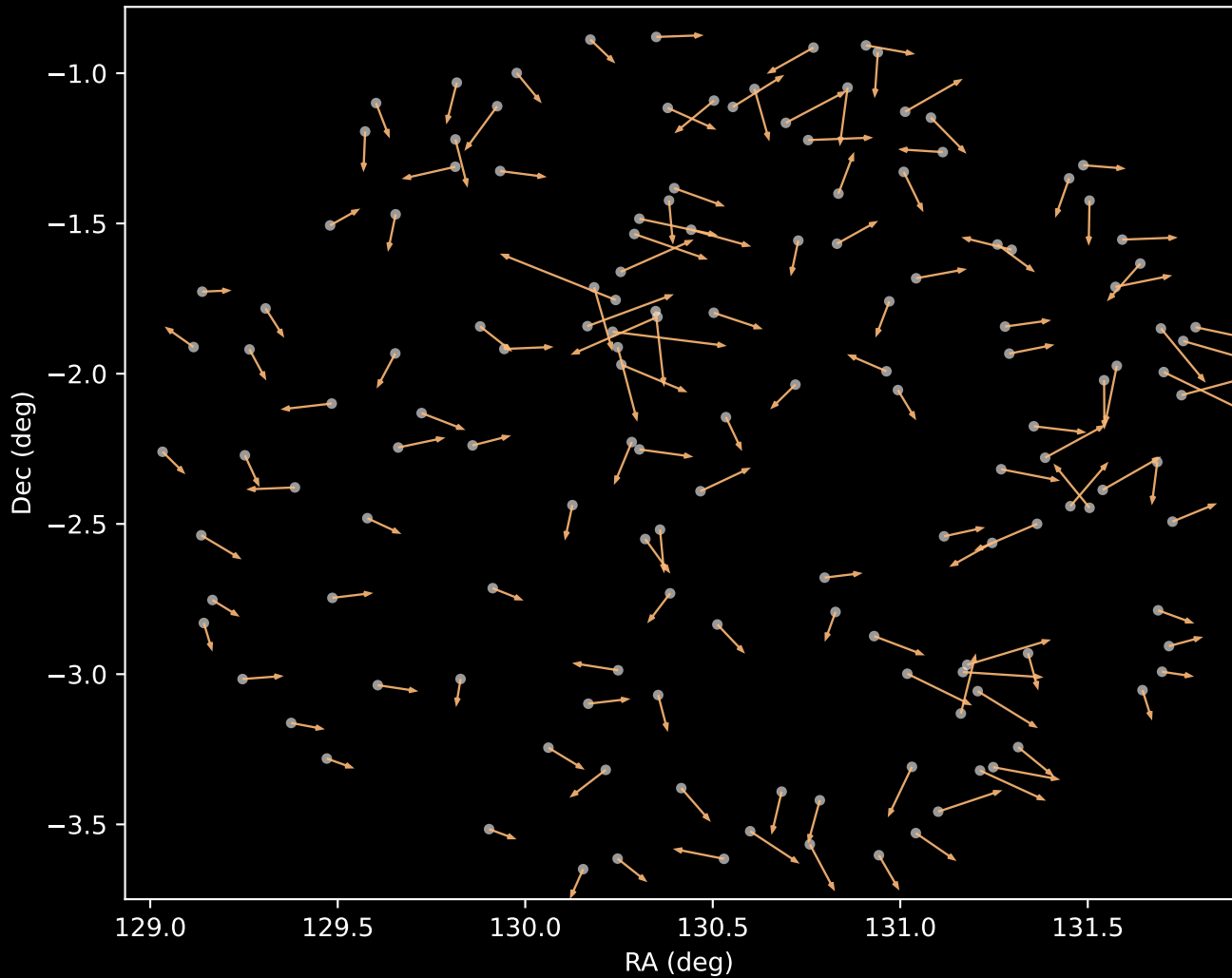
APOGEE DR17 Cluster 3 Proper Motion Vectors (n=145)
