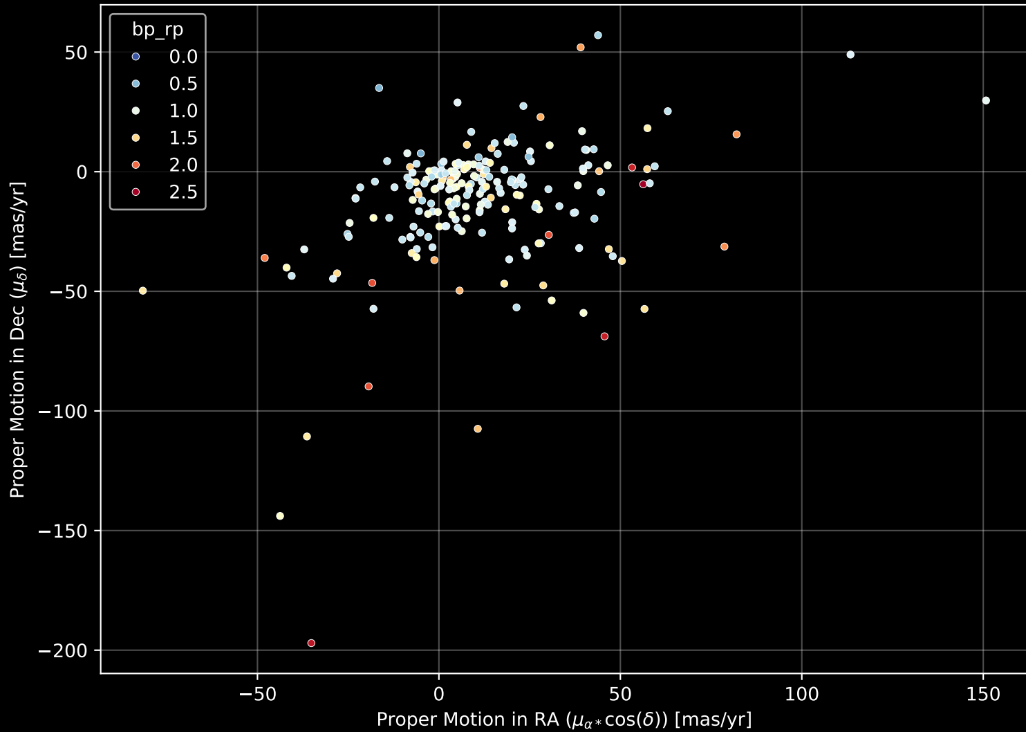
APOGEE DR17 Field: [160-60] Proper Motion Diagram (n= 219)
